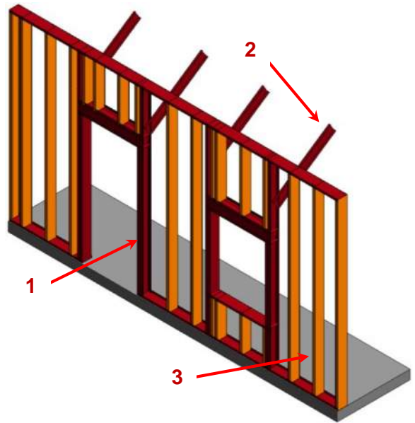
81 C1010.05-LOD-350 Interior Wall (Cold-Form Metal Framing)
